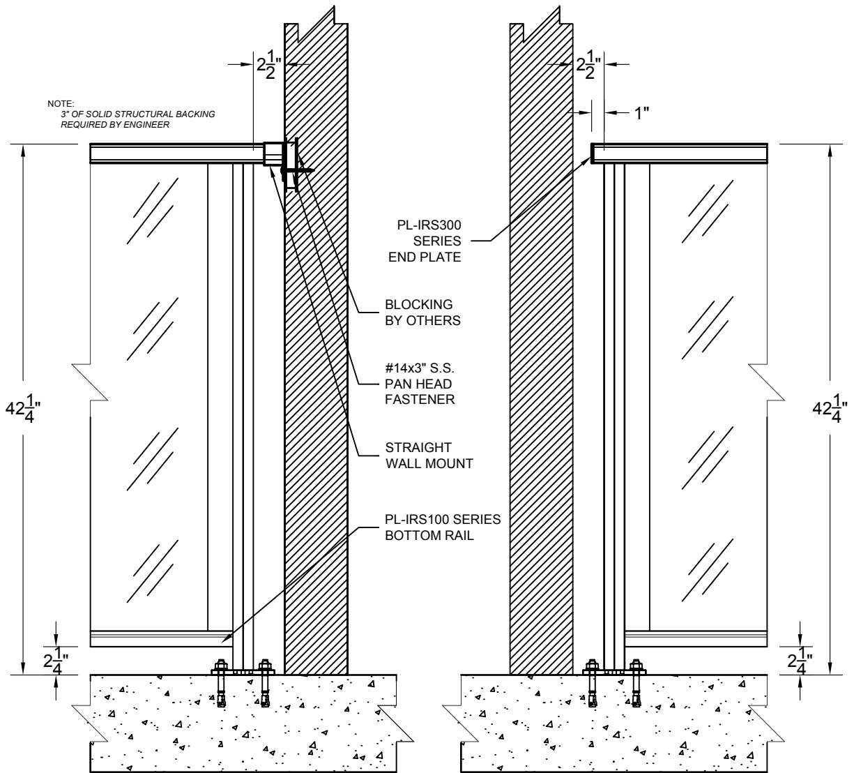
WALL MOUNTING DETAIL
